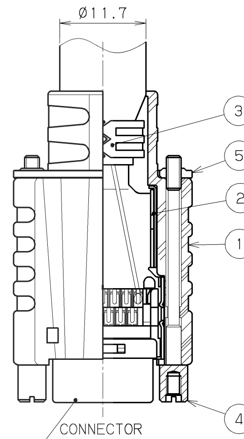
AFTER ASSEMBLY DRAWING
