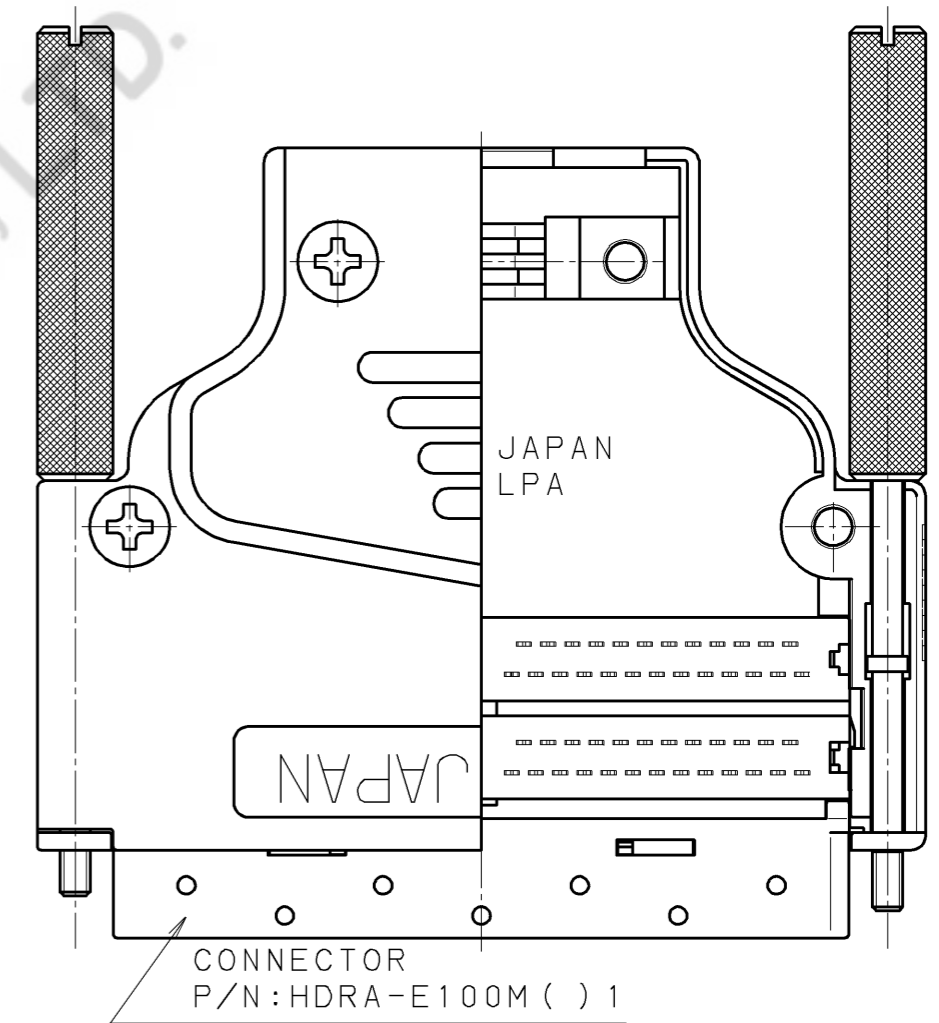
△ DRAWING AFTER CONNECTOR ASSEMBLY
